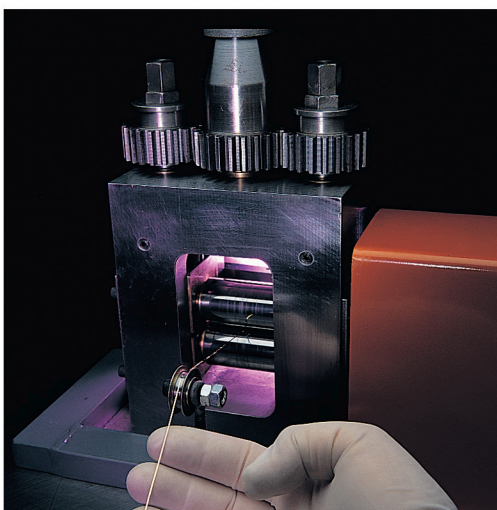
Precious metal rolling mill custom-built and specifically designed for fabrication of gold, silver, and platinum ribbon. Dimensional tolerances as tight as .00015".
